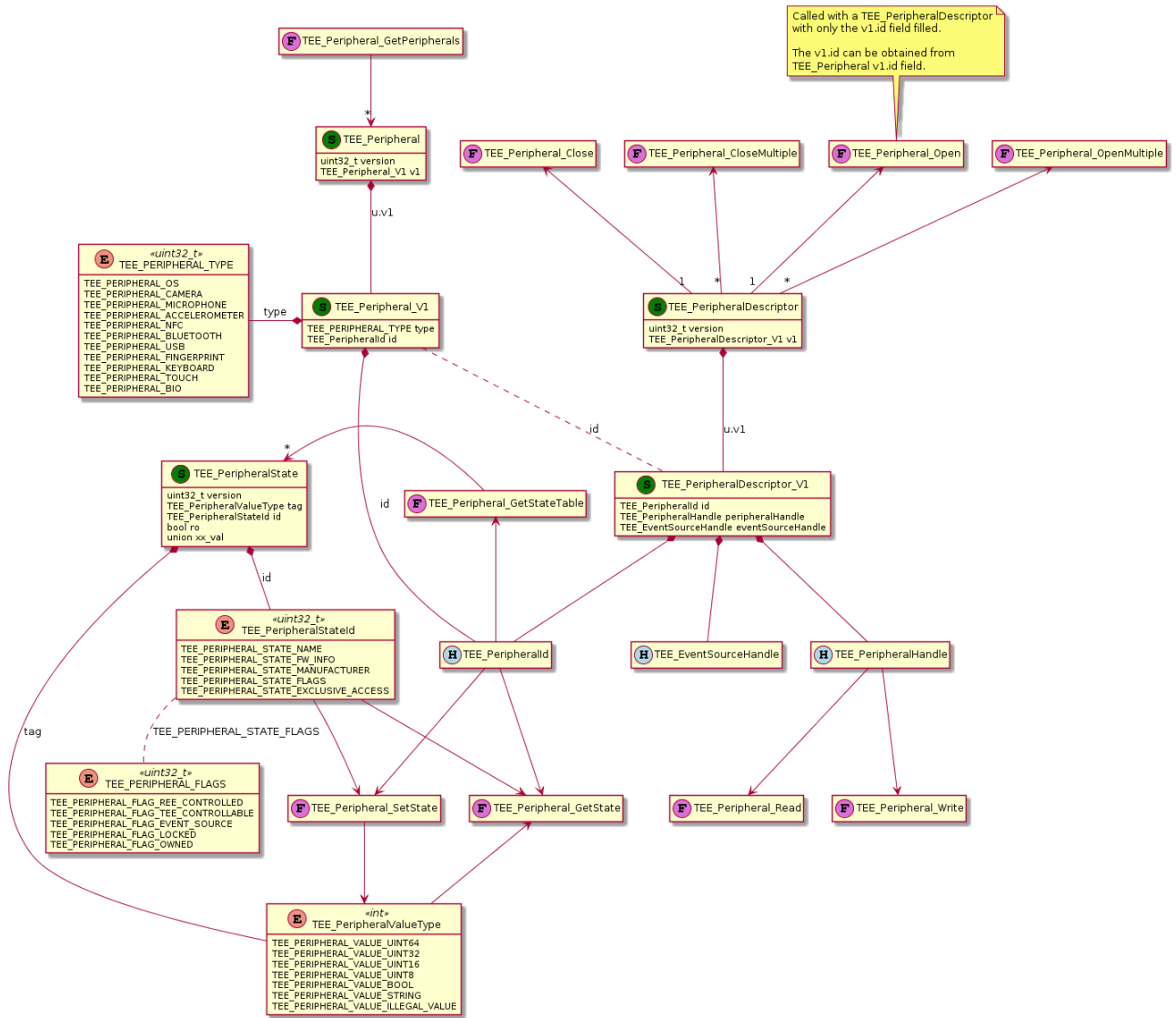
Figure 9-2: Peripheral API Overview
