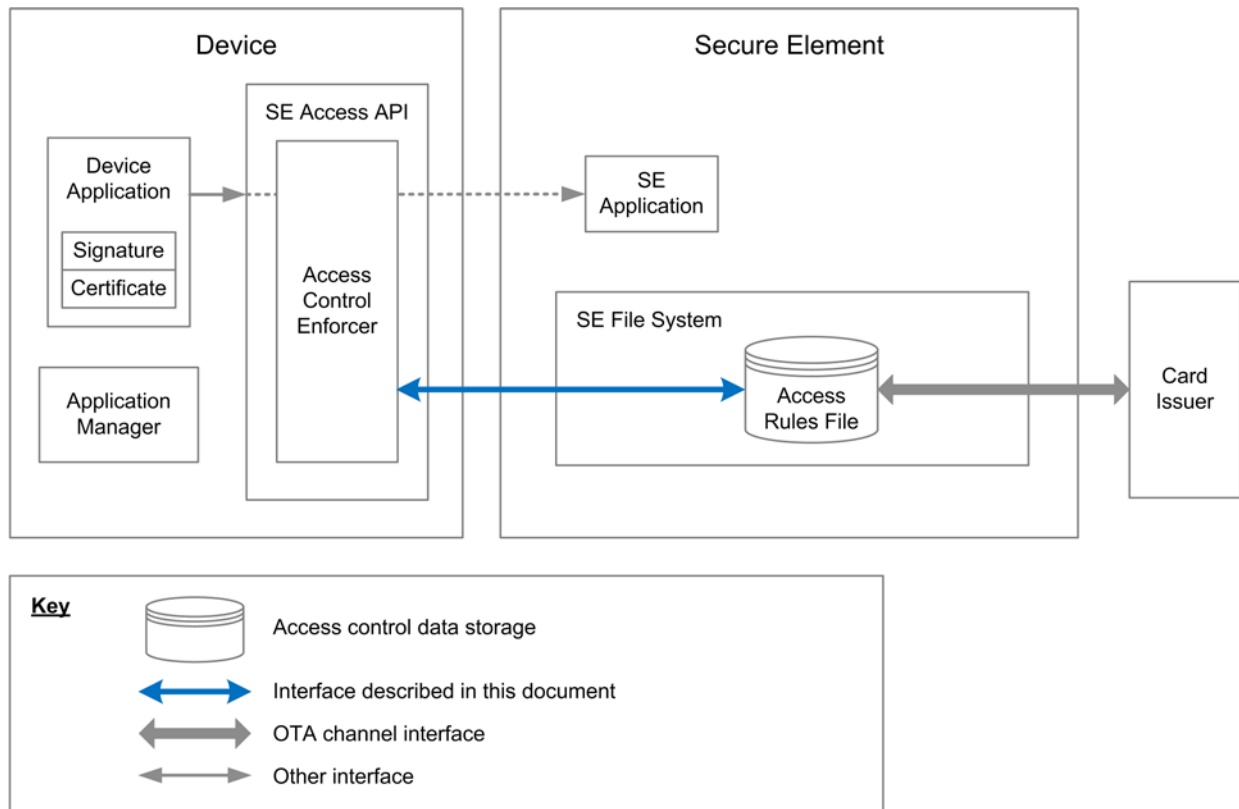
Figure 2-4: Access Control Architecture with Access Rules File System Fallback
