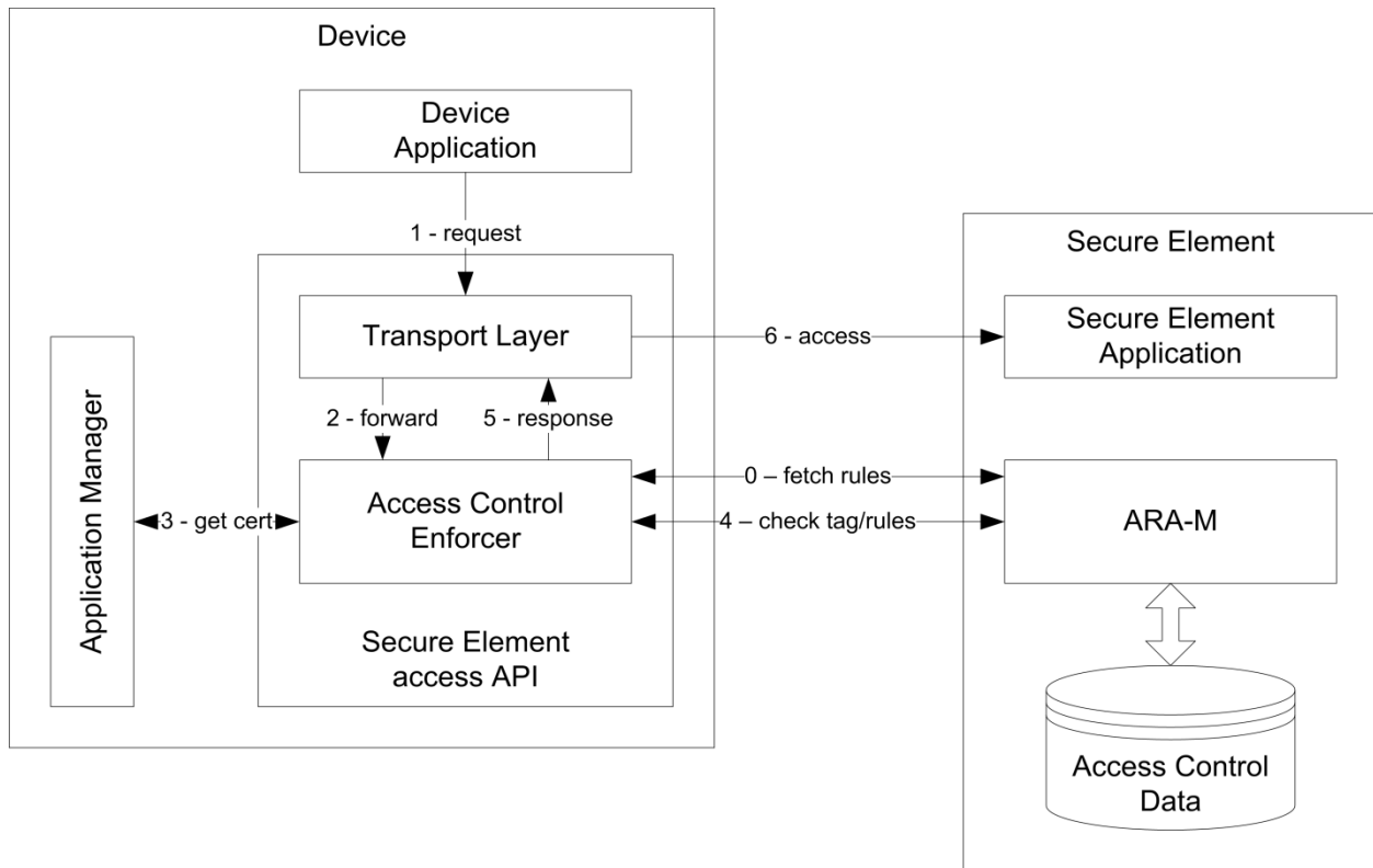
Figure 4-1: Device Interface Sequence with Rules Caching
