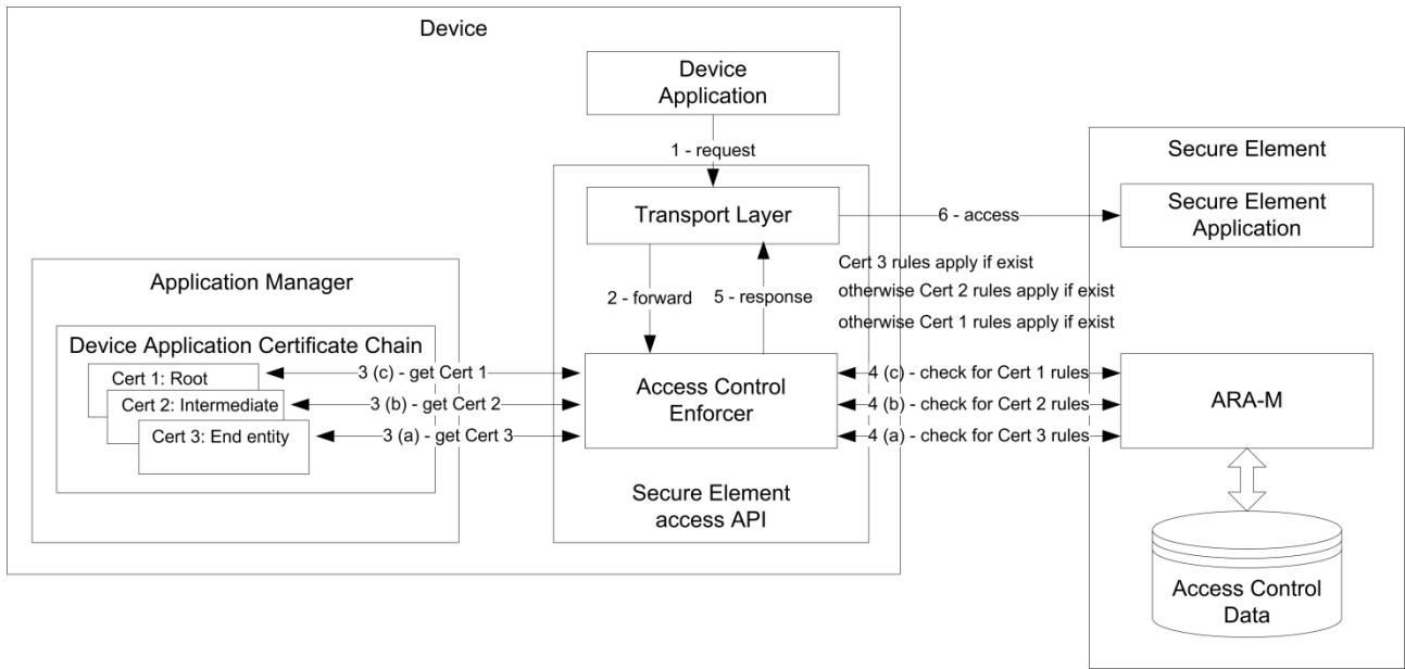
Figure 4-3: Processing of Chained Certificates
